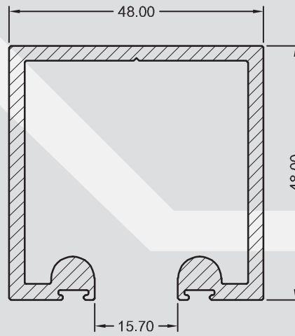
SP-4848 1,435 KG/M
